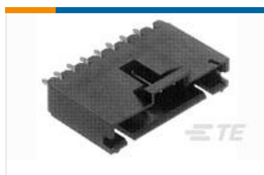
TE 系列/零件编号5-103735-5 06 MTE HDR SRST LATCH .100CL
