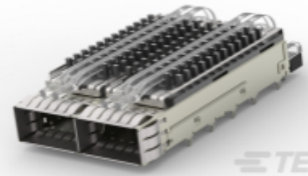
TE 系列/零件编号2-2170808-5 QSFP28, 1X2, CAGE ASSY, SPRING, HS, LP
