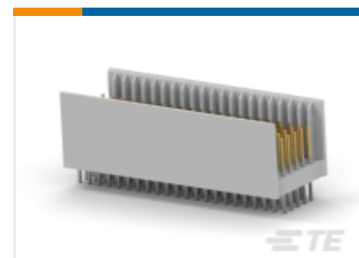
TE 系列/零件编号 5352132-1 Z-PACK/B MALE HDR 110P
