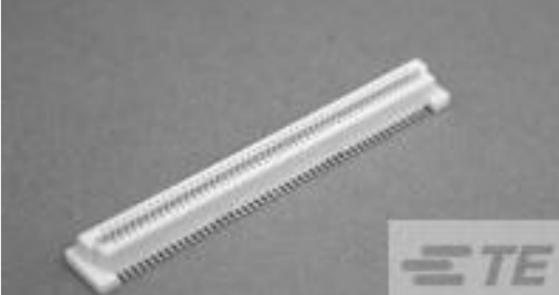
TE 系列/零件编号1- 5353999-0 0.8FH,R05H.5,200,30/Sn, TR,SC
