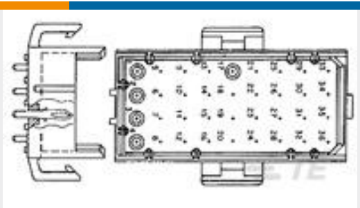
TE 系列/零件编号640499-4 04P MR HDR ASSY V0 RED
