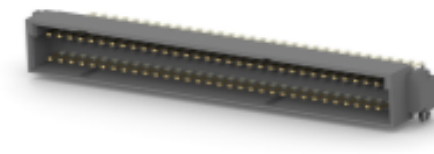
TE 系列/零件编号 5536356-5 ASSY,PIN,EUROCARD,"C", LEAD-FREE,A&C,64/9
