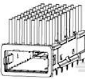
TE 系列/零件编号1888065-1 XFP Networking Kit(cage, clip, heatsink)
