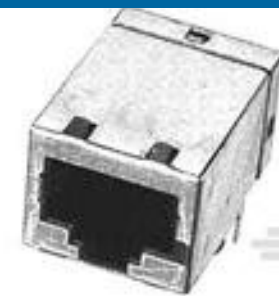
TE 系列/零件编号1- 1734264-3 M/J,RJ45,Side,8P8C,R/A, 50u" Au, D3.2
