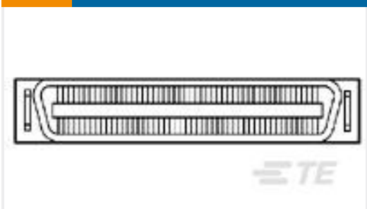
TE 零件编号6-5175473-0 .050CL,CHAMP,VERT PLUG,100 POS
