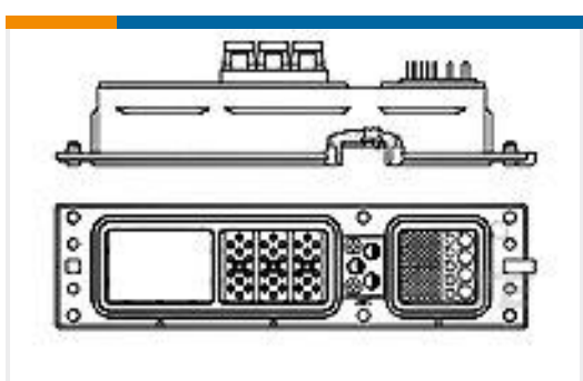
TE 零件编号1883150-2 A600 SZ 2 RCPT F36/blnk /59
