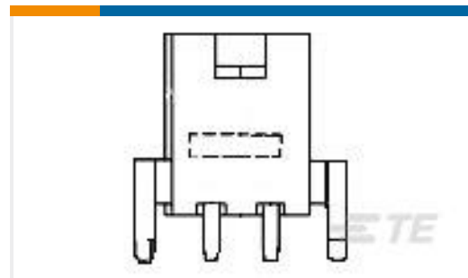
TE 零件编号292323-1 REC ASSY RIGHT ANGLE STACKED THRUHOLE US
